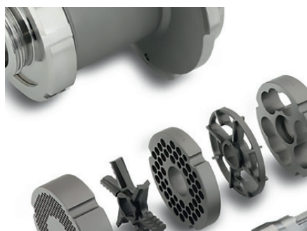
Sausage grinder980 with separation function
